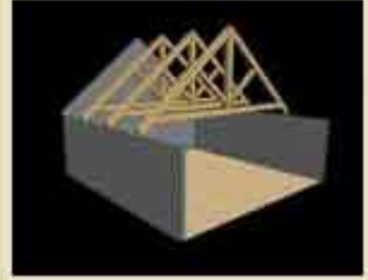
Raised Chord King Post With Struts
