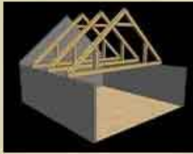
Collar Tie With Queen Post
