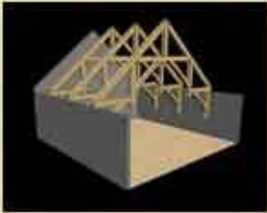
Hammerbeam
